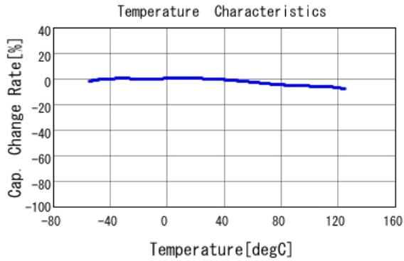
■ GCD188R71H223KA01 C-Temp. capchange, DC0.0V, AC1.0Vrm
