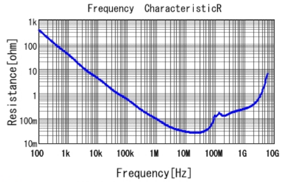
GCD188R71H223KA01 R DCOV, 25degC
