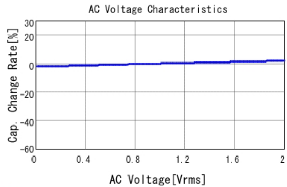
GCD188R71H223KA01 C-AC Voltage capchange, DCOV, 25.0d
