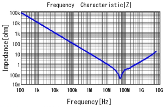
GCD188R71H223KA01 |Z| DCOV, 25degC
