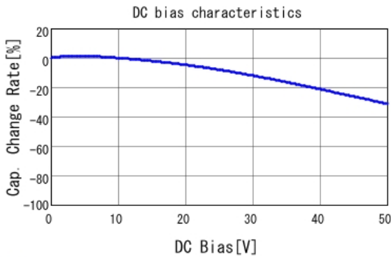
GCD188R71H223KA01 C-DC bias capchange, 25.0degC, AC1.
