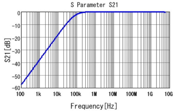
■ GCD188R71H223KA01 S21 DC0V, 25degC
