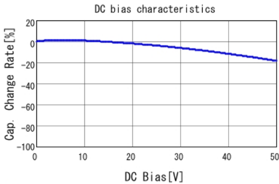
■ GCD188R71H103MA01 C-DC bias capchange, 25.0degC, AC1.
