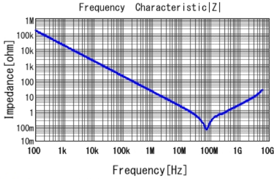
■ GCD188R71H103MA01 |Z| DCOV, 25degC
