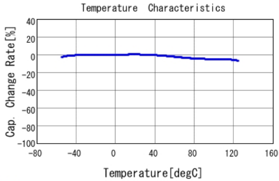
■ GCD188R71H103MA01 C-Temp. capchange, DC0.0V, AC1.0Vrm
