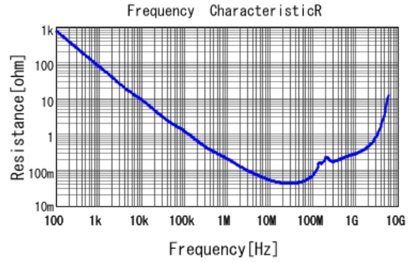
■ GCD188R71H103MA01 R DCOV, 25degC
