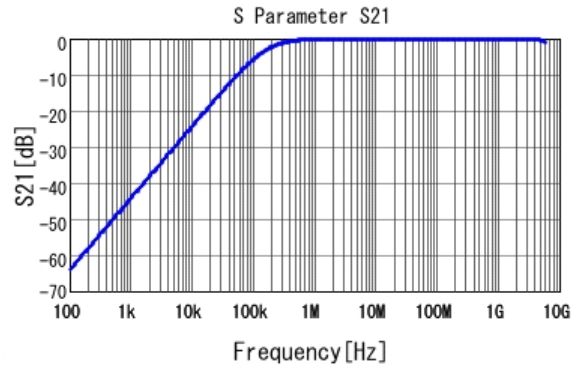
■ GCD188R71H103MA01 S21 DC0V, 25degC
