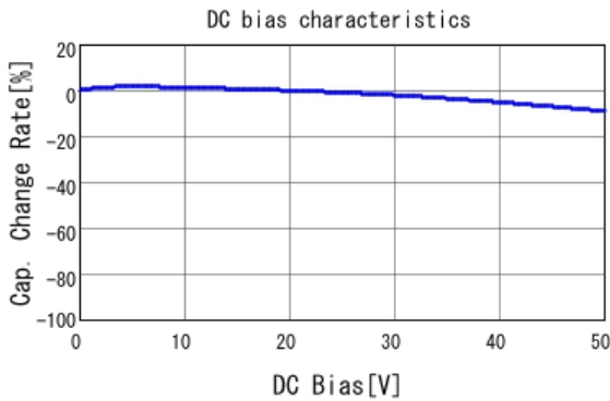
GCD188R71H102MA01 C-DC bias capchange, 25.0degC, AC1.
