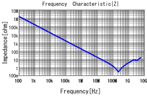
GCD188R71H102MA01 |Z| DCOV, 25degC
