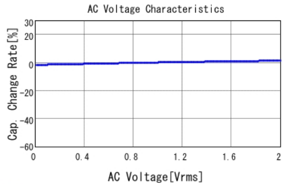
GCD188R71H102MA01 C-AC Voltage capchange, DCOV, 25.0d
