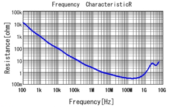
GCD188R71H102MA01 R DCOV, 25degC
