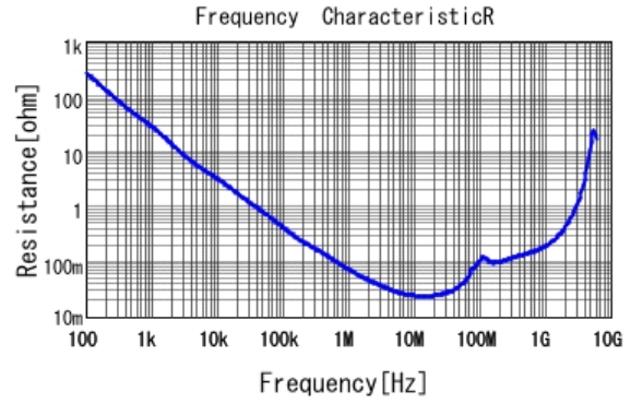
■ GCD188R71E333KA01 R DCOV, 25degC
