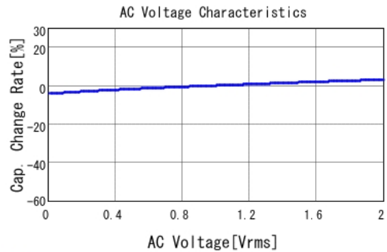
■ GCD188R71E333KA01 C-AC Voltage capchange, DCOV, 25.0d
