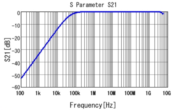
■ GCD188R71E333KA01 S21 DC0V, 25degC
