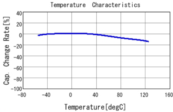
■ GCD188R71E333KA01 C-Temp. capchange, DC0.0V, AC1.0Vrm
