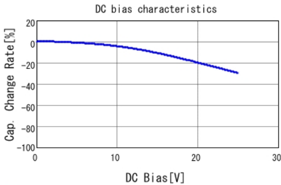
■ GCD188R71E333KA01 C-DC bias capchange, 25.0degC, AC1.
