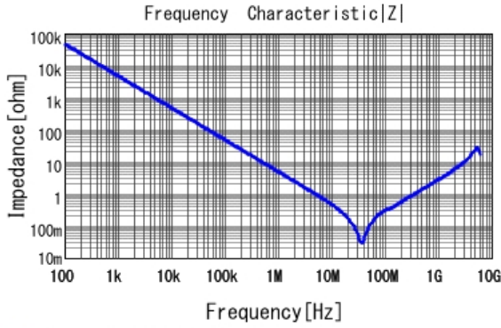
■ GCD188R71E333KA01 |Z| DCOV, 25degC
