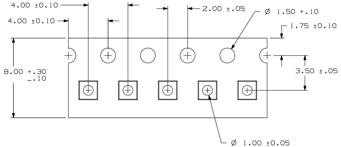
Figure 23 • Tape-and-Reel Format
