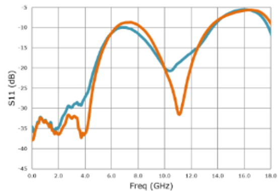
Figure 7 • GC4212-6LP/GC4701-6LP/GC9952-6LP Input Return Loss
