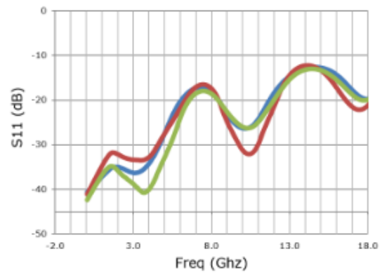
Figure 5 • GC4212-6LP/GC4701-6LP Input Return Loss
