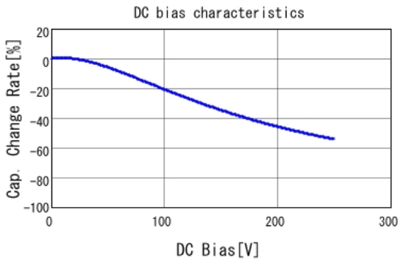
■ GC331AD72E333KX01 C-DC bias capchange, 25.0degC, AC1V
