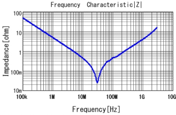
■ GC331AD72E333KX01 |Z| DC0V, 25degC
