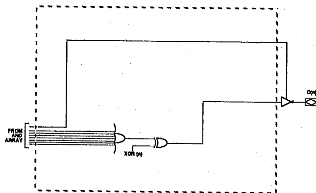
Combinational Output with Programmable OE and Polarity
