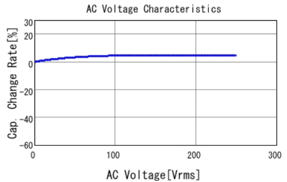
■ GA352QR7GF101KW31 C-AC Voltage capchange, DCOV, 25.0d
