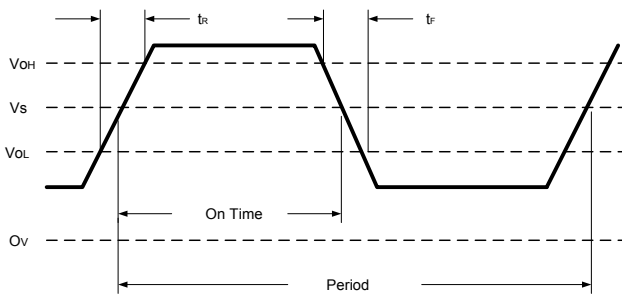
FIGURE 2. Output Waveform
