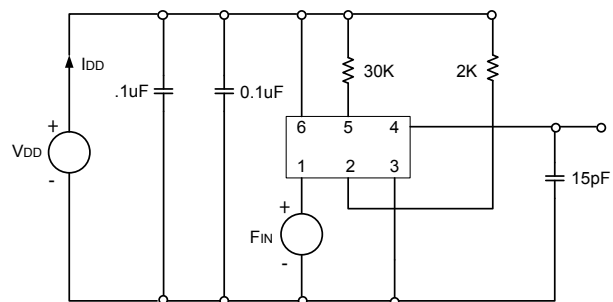
Figure 3. Output Test Conditions (25 ± 5°C)
