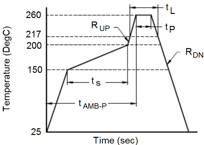
Figure 4. Suggested IR Profile
