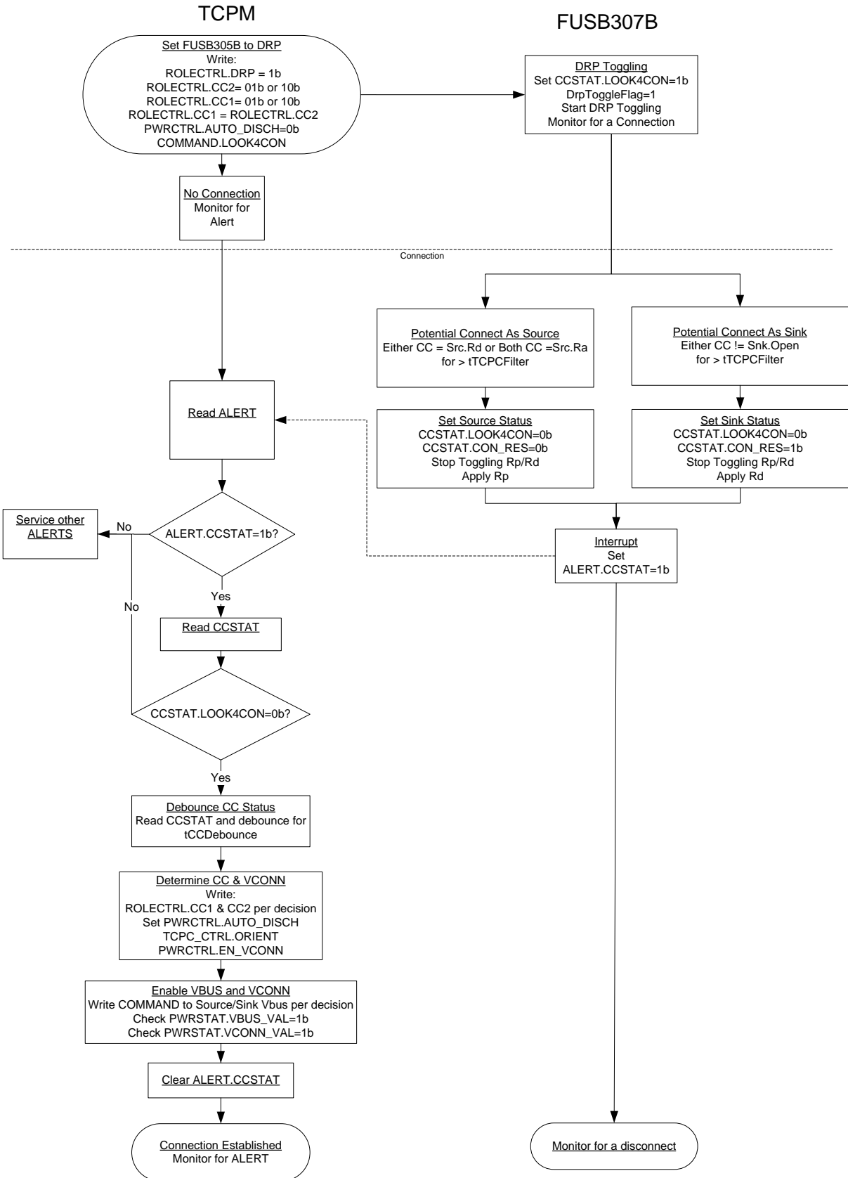
Figure 9. DRP Initialization and Connection Detection
