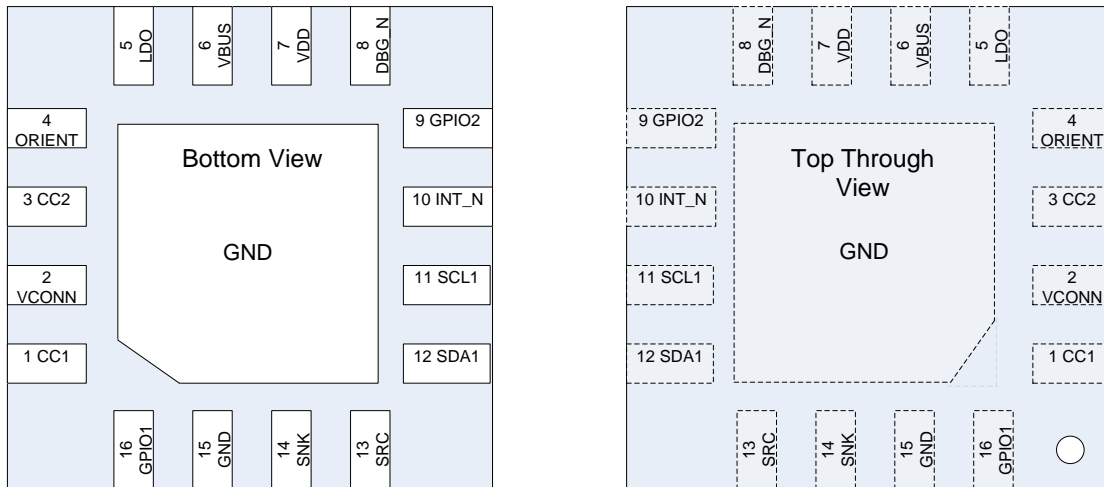
Figure 5. Pin Assignment QFN (FUSB307B)
