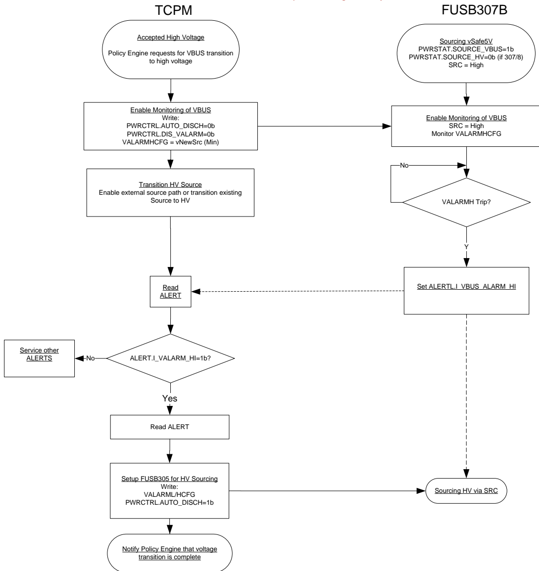
Figure 14. Transition to High Voltage using SRC Controlled Path VBUS
