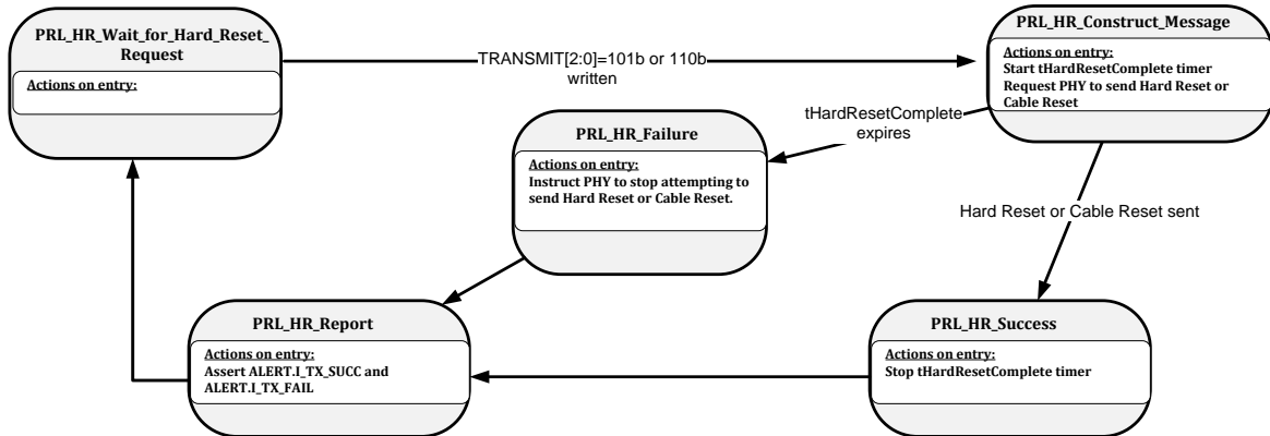
Figure 12. Hard Reset and Cable Reset State Machine
