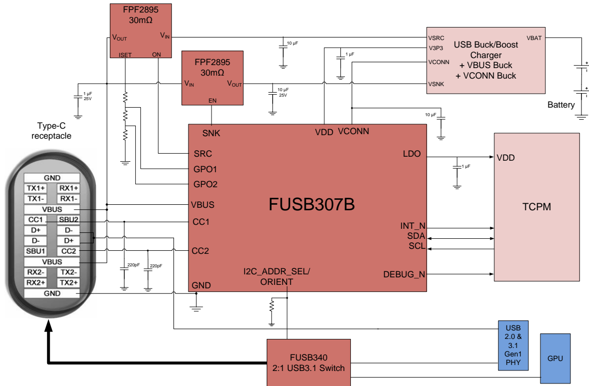
Figure 3. FUSB307B Typical Mobile Computing Application
