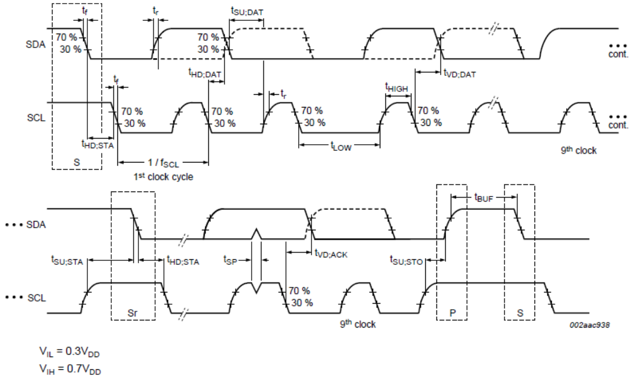
Figure 20. Definition of Timing for Full-Speed Mode Devices on the I2C Bus
