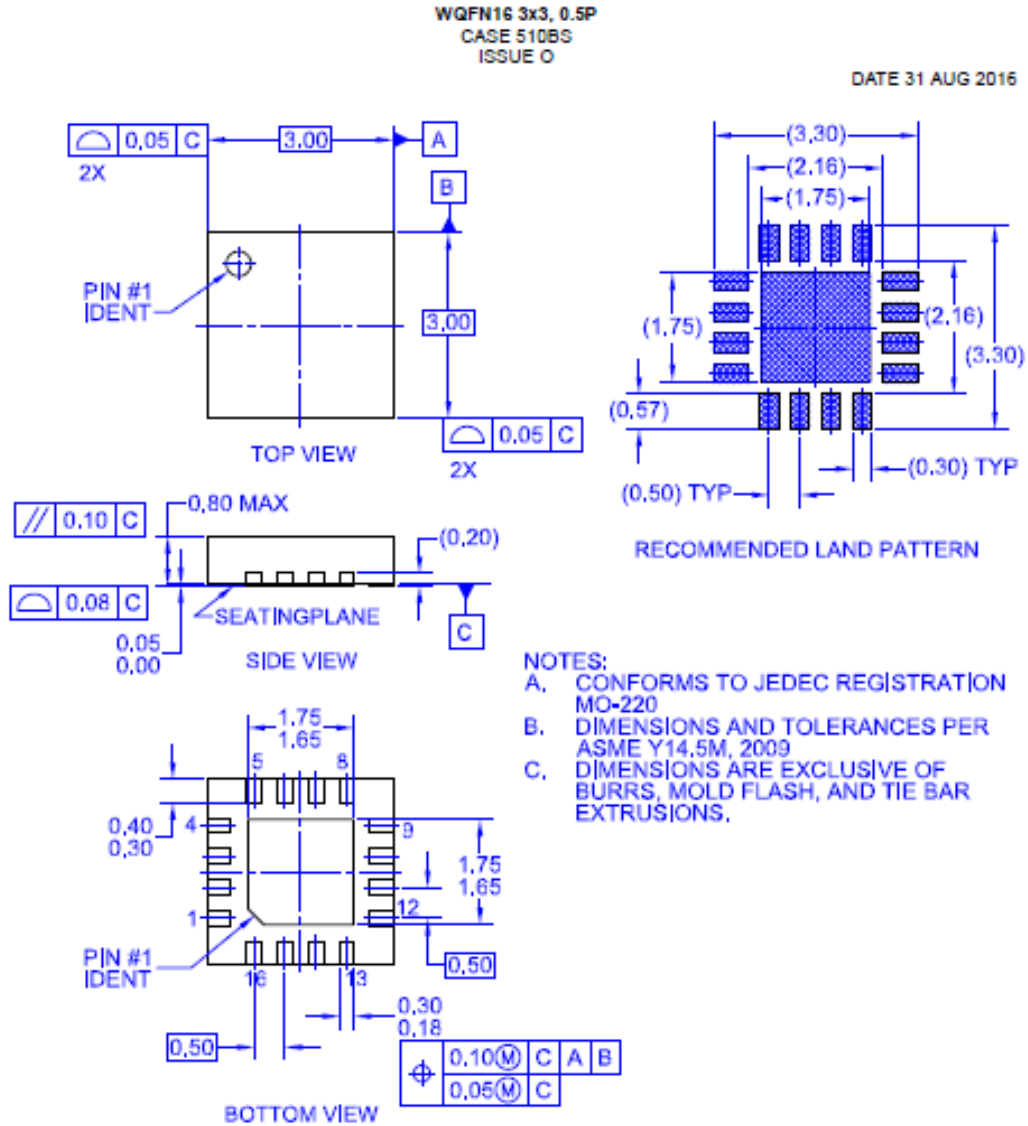
Figure 21. 16-lead Molded Leadless Package (QFN) JEDEC, ML220, 3 mm Square
