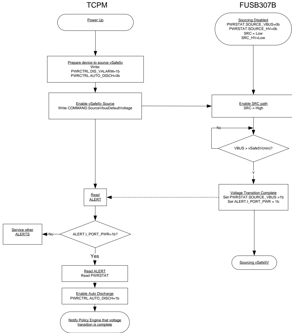
Figure 13. Transition to vSafe5V on Power Up
