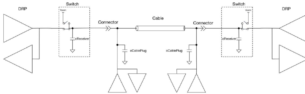
Figure 19. Transmitter Test Load
