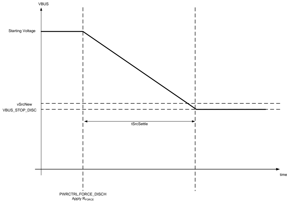
Figure 17. Source Discharge during a Connection
