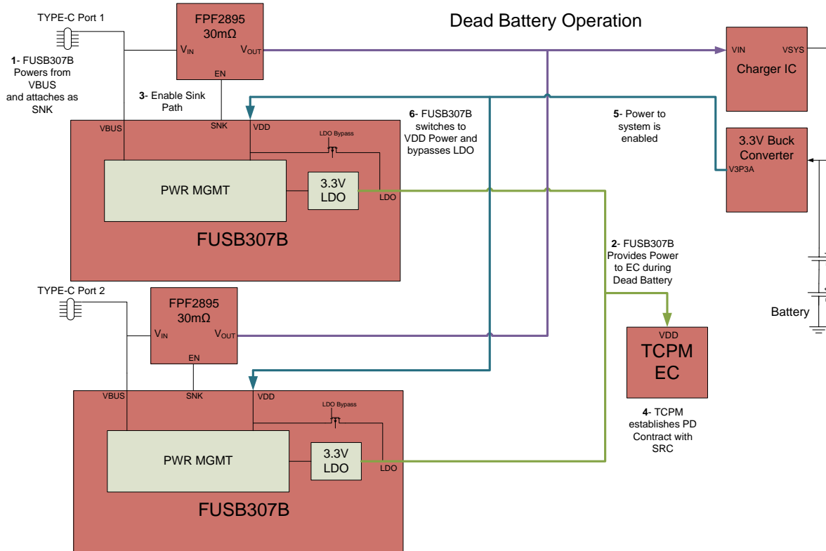
Figure 6. FUSB307B Dead Battery Operation
