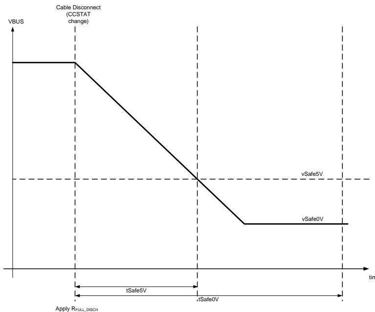
Figure 15. VBUS Auto Discharge as Source
