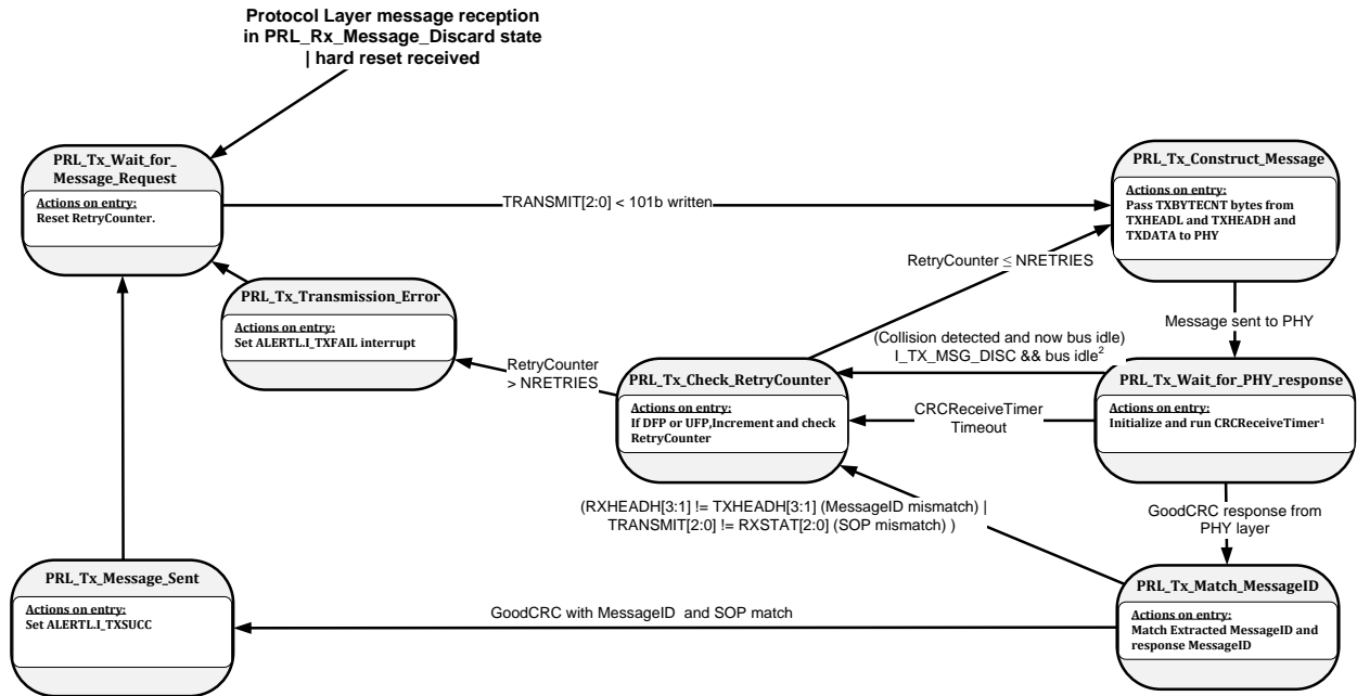
Figure 11. Transmit State Machine
