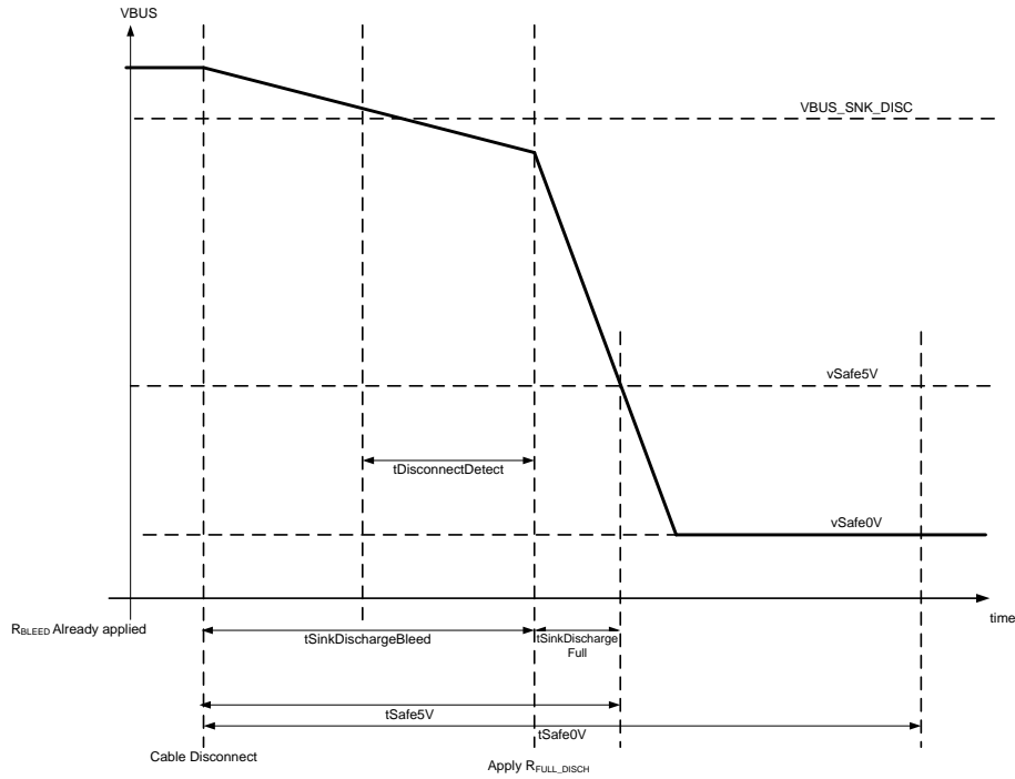
Figure 16. VBUS Auto Discharge as SinkSource
