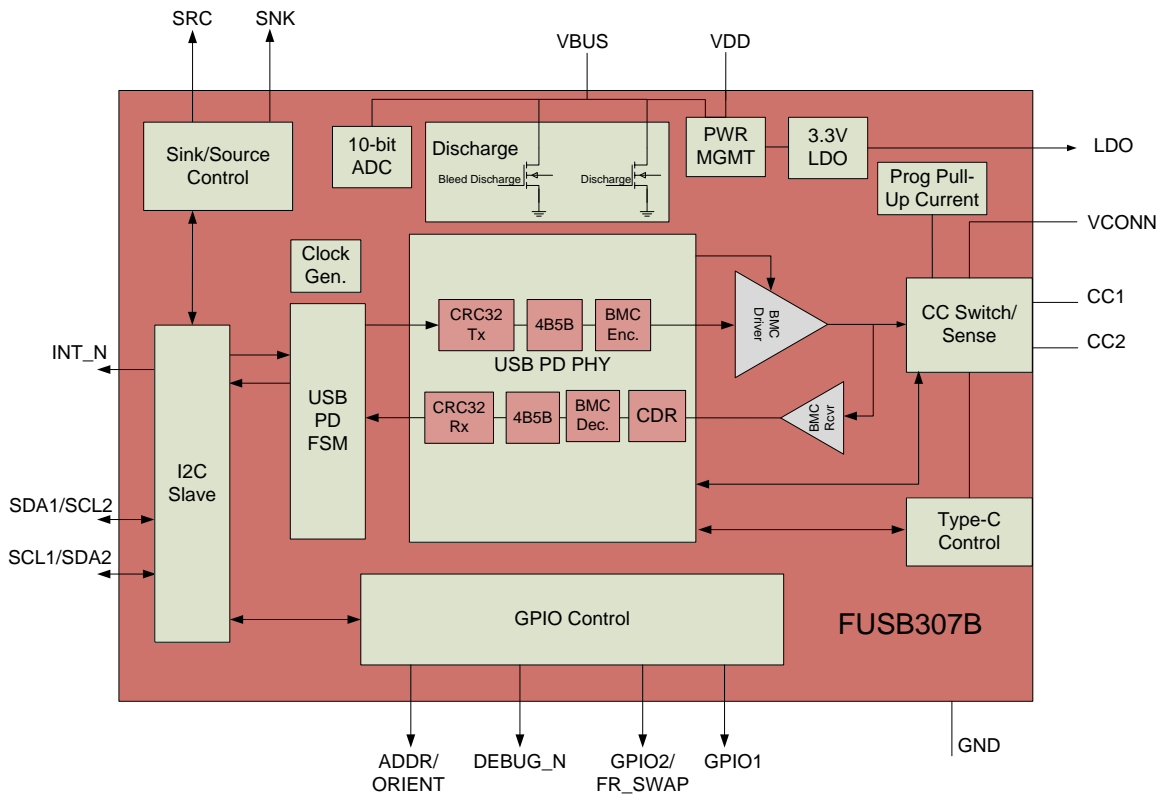
Figure 4. FUSB307B Block Diagram
