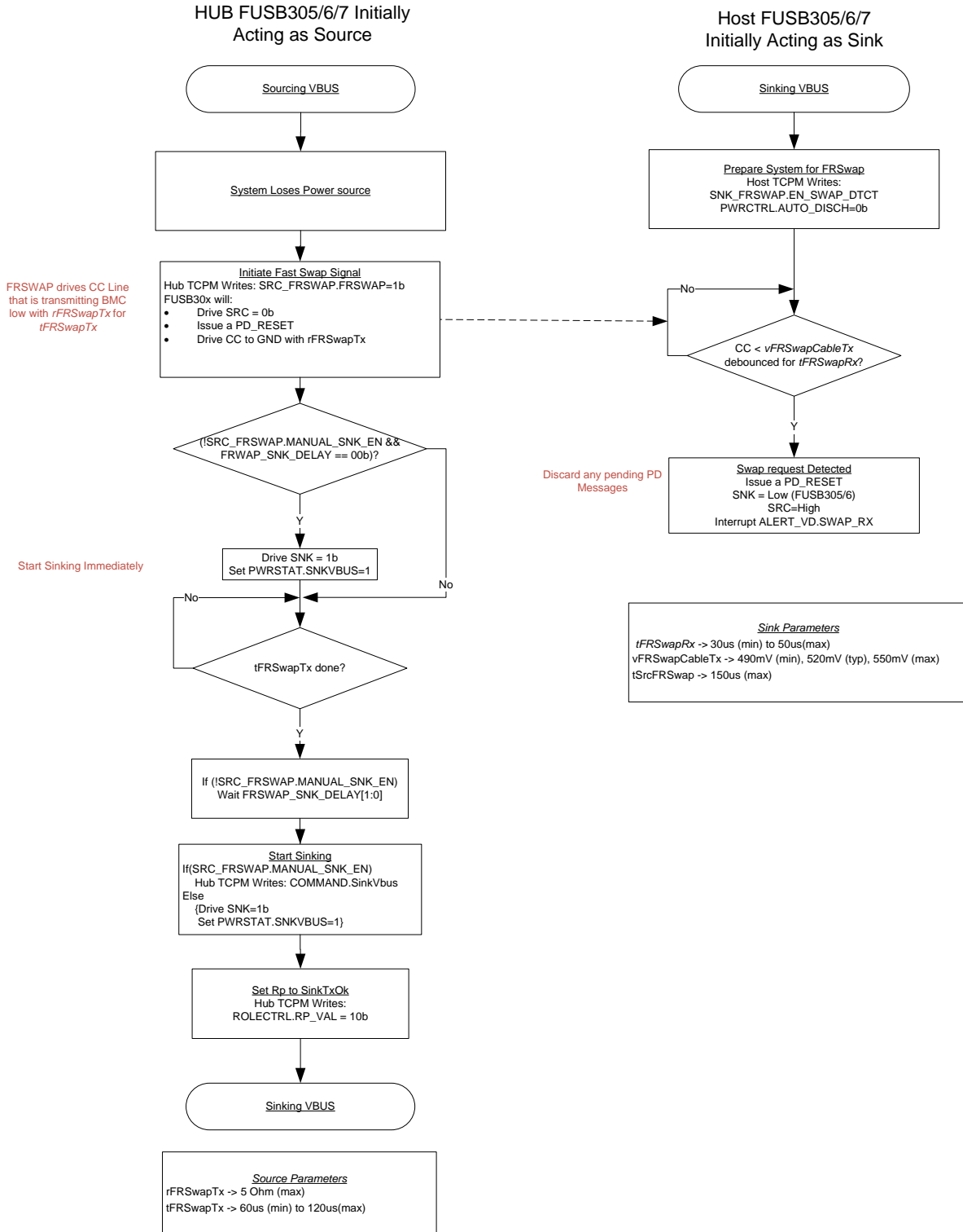
Figure 18. Fast Role Swap Flow Diagram
