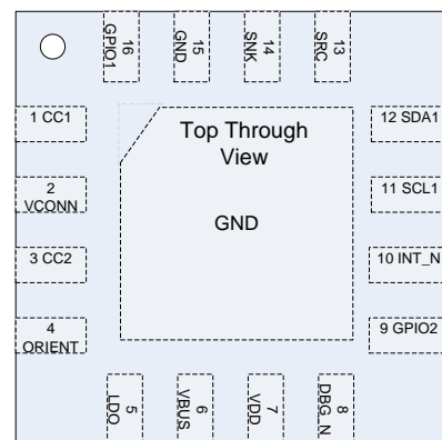
Figure 2. QFN16
