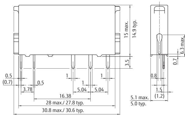
Socket type
