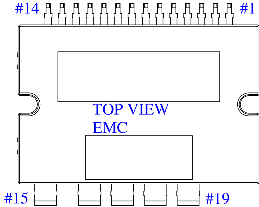
Figure 1. Pin Configuration
