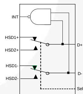
Figure 1. Analog Symbol
