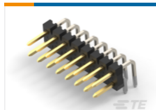
TE Part #5-2823140-0 50P,2MM,BRK HDR,DRRT,2,8,0.76AU, TB
