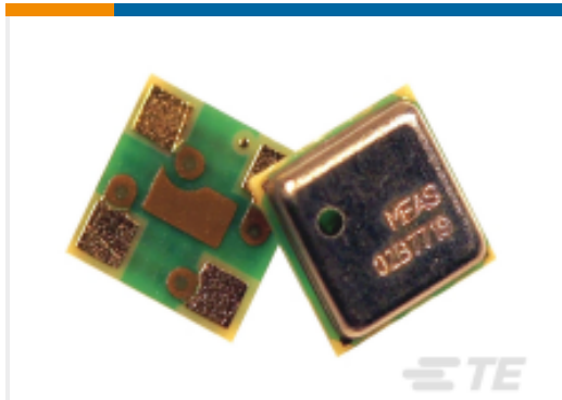
TE Part #MS563702BA03-50 2 BAR INDUSTRIAL ALTIMETER SENSOR
