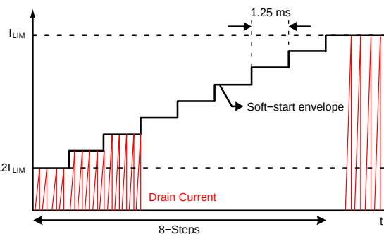
Figure 27. Internal Soft-Start
