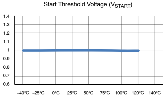
Figure 7. Start Threshold Voltage vs. Temperature
