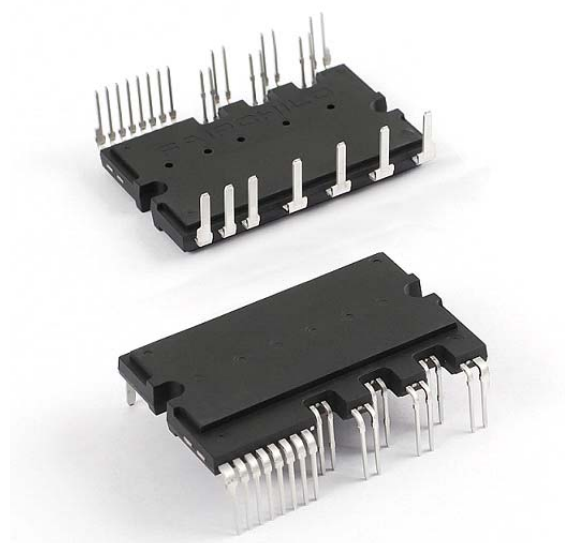
Figure 1. Package Overview
