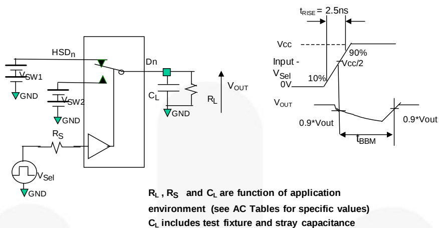
Figure 10. Break-Before-Make Interval Timing
