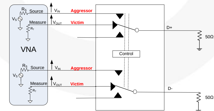
Figure 12. Non-Adjacent Channel-to-Channel Crosstalk (SDD21)
