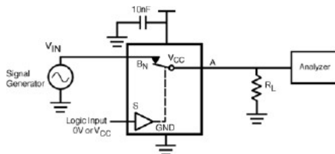
Figure 9. Harmonic Distortion
