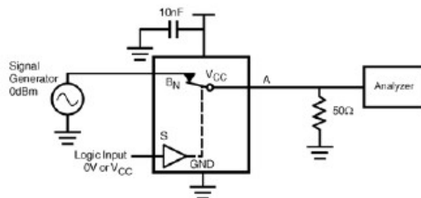
Figure 8. Bandwidth
