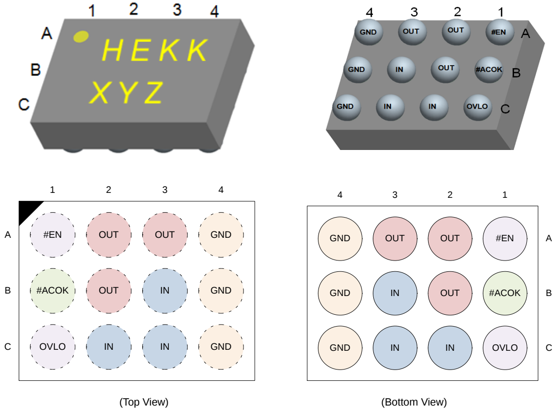
Figure 2. Pin Configuration
