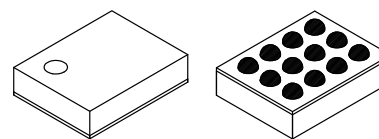
WLCSP12 1.288x1.828x0.586 CASE 567QX
