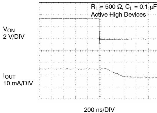
Figure 21. T OFF Response
