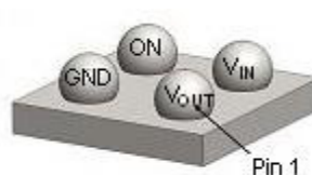
Figure 4. 1 x 1 mm WLCSP Bumps Facing Up
