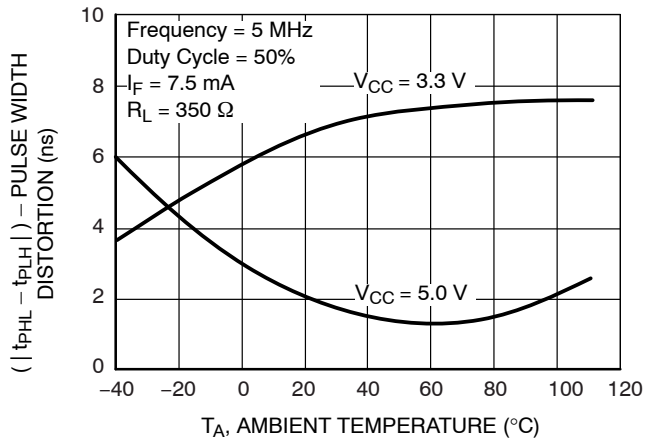
Figure 9. Typical Pulse Width Distortion vs. Ambient Temperature
