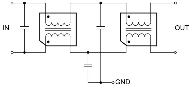
Figure 4. Internal Schematic
