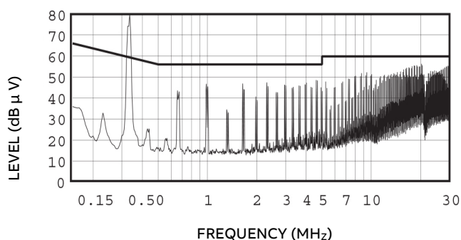
Figure 10. JAW075A1 Conducted Noise with Filter Compared to Class B Limits
