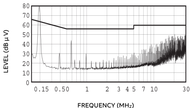
Figure 9. HW050FG Conducted Noise with Filter Compared to Class B Limits
