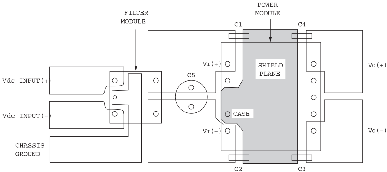
Figure 5. Recommended Schematic When Used as the Input Filter to a High-Frequency dc-to-dc Converter
