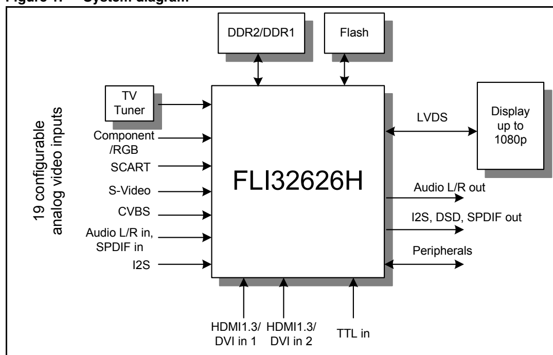
Figure 1. System diagram
