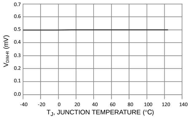
Figure 11. V DIM-R vs. Temperature
