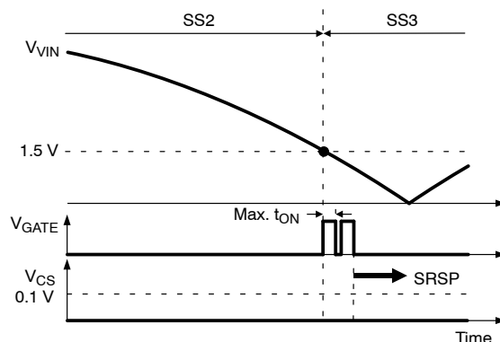
Figure 21. Sensing resistor Short Protection
