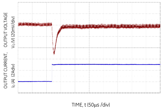
Figure 22. Transient Response to Dynamic Load Change from 50% to 100% at 12Vin, C_{out}=5\times 100\mu\text{F} , C_{tune}=3.3\text{nF} , R_{tune}=500
