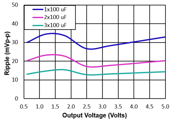
Figure 38. Output ripple voltage for various output voltages with external 1x100 \mu F, 2x100 \mu F, and 3x100 \mu F ceramic capacitors at the output (6A load). Input voltage is 12V.
