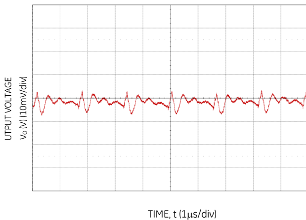
Figure 3. Typical output ripple and noise ( C_o=88\mu\text{F} ceramic, V_{IN} = 12\text{V} , I_o = I_{o,max} ).
