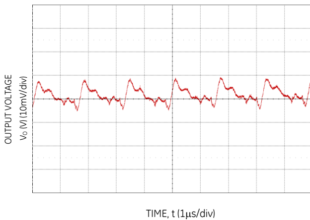
Figure 21. Typical output ripple and noise ( C_o=88\mu\text{F} ceramic, V_{IN} = 12\text{V} , I_o = I_{o,max} ).
