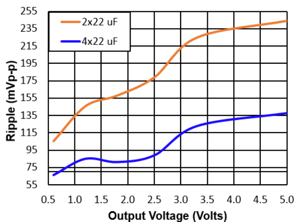
Figure 37. Input ripple voltage for various output voltages with 2x22 \mu F or 4x22 \mu F ceramic capacitors at the input (6A load). Input voltage is 12V.
