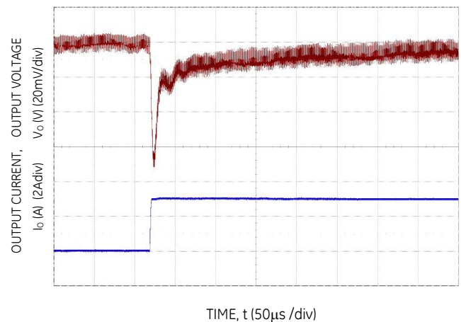
Figure 34. Transient Response to Dynamic Load Change from 50% to 100% at 12Vin, C_{out}=3 \times 100\mu\text{F} , C_{tune}=1.5\text{nF} , R_{tune}=500
