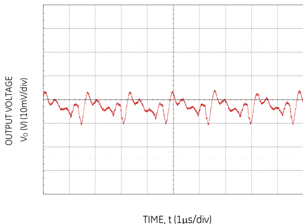
Figure 15. Typical output ripple and noise ( C_o=88\mu\text{F} ceramic, V_{IN} = 12\text{V} , I_o = I_{o,max} ).
