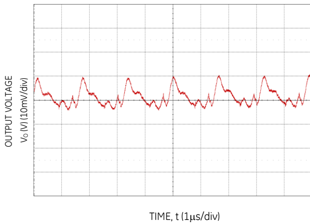
Figure 27. Typical output ripple and noise ( C_o=88\mu\text{F} ceramic, V_{IN} = 12\text{V} , I_o = I_{o,max} ).
