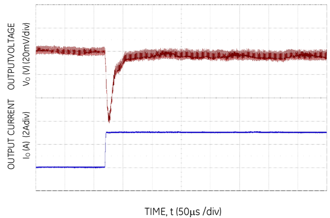
Figure 28. Transient Response to Dynamic Load Change from 50% to 100% at 12Vin, C_{out}=4\times 100\mu\text{F} , C_{tune}=2.2\text{nF} , R_{tune}=500
