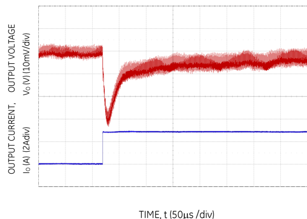
Figure 16. Transient Response to Dynamic Load Change from 50% to 100% at 12V in , C_{out}=1\times 330\mu\text{F} , 4\times 100\mu\text{F} , C_{tune}=4.7\text{nF} , R_{tune}=500
