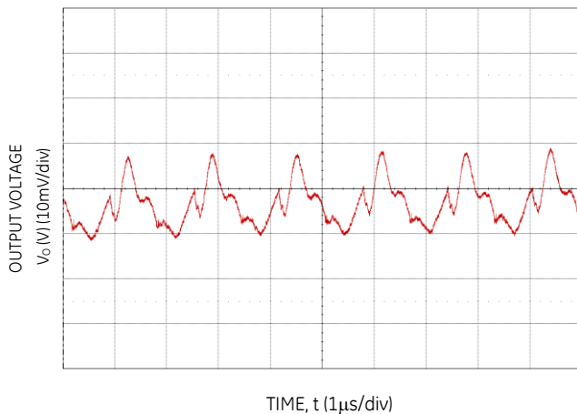
Figure 33. Typical output ripple and noise ( C_o=88\mu\text{F} ceramic, V_{IN} = 12\text{V} , I_o = I_{o,max} ).
