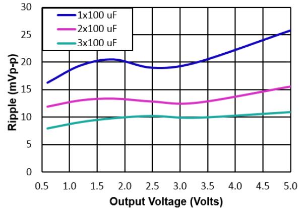
Figure 38. Output ripple voltage for various output voltages with external 1x100µF, 2x100µF, and 3x100µF ceramic capacitors at the output (3A load). Input voltage is 12V.
