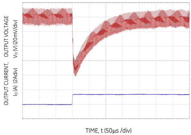
Figure 34. Transient Response to Dynamic Load Change from 50% to 100% at 12Vin, C_{out}=1\times 100\mu\text{F} , C_{tune}=680\text{pF} , R_{tune}=500
