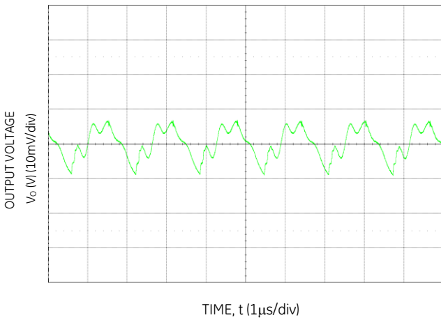
Figure 33. Typical output ripple and noise ( C_o=88\mu\text{F} ceramic, V_{IN} = 12\text{V} , I_o = I_{o,max} ).
