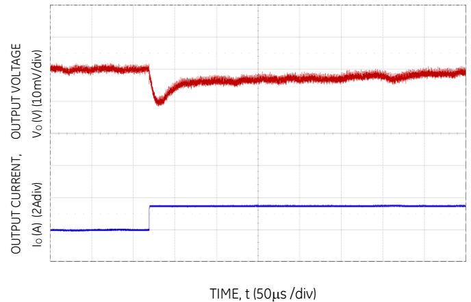
Figure 4. Transient Response to Dynamic Load Change from 50% to 100% at 12V in , C out -2x330µF, 6x100µF, C tune -10nF, R tune -500
