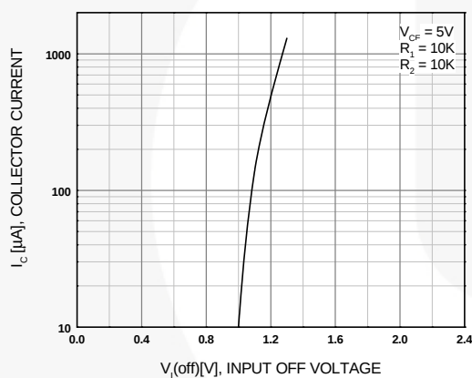
Figure 3. Input-Off Voltage
