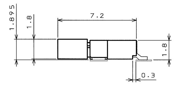
MATED CONDITION (REF.) 嵌合状態図 (参考)
