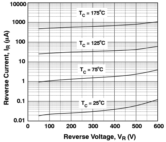
Figure 22. Reverse Current
