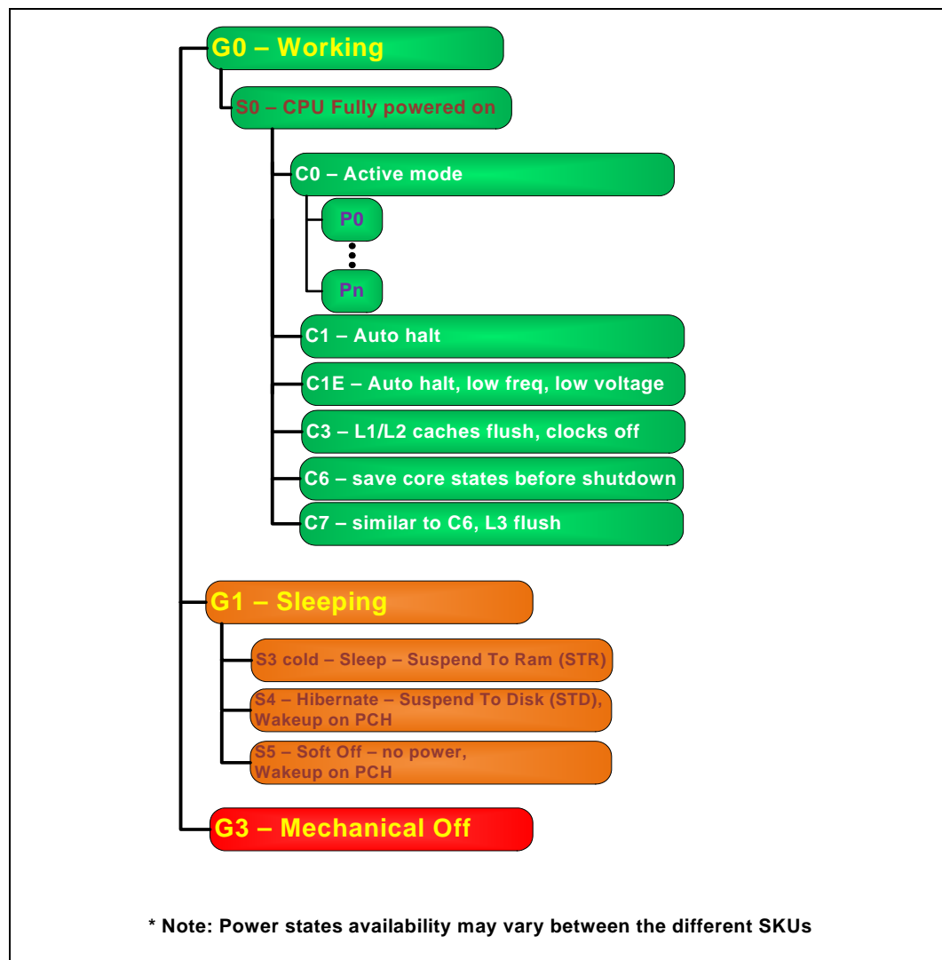
Figure 4-1. Power States
