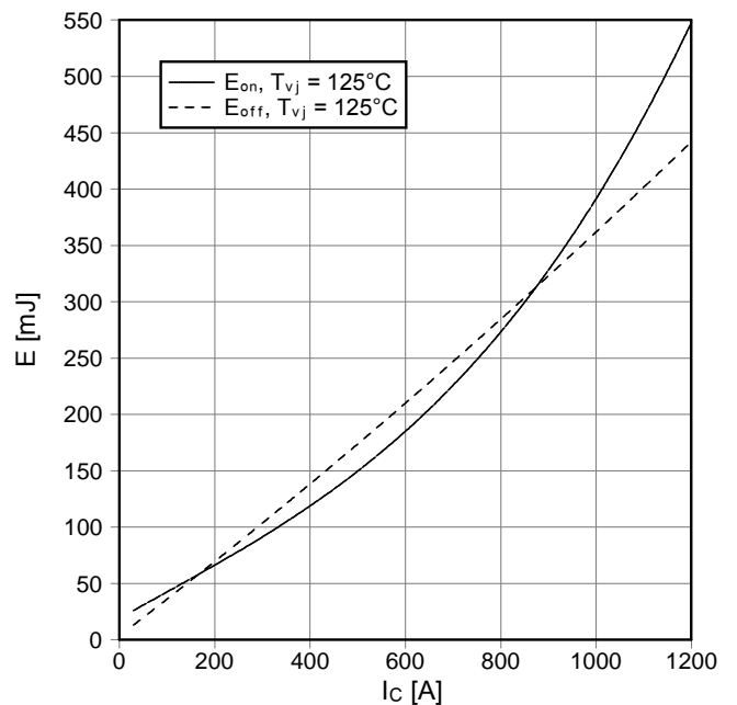
Schaltverluste IGBT- Wechslr. (typisch) switching losses IGBT-inverter (typical)- E_{on} = f(I_C) , E_{off} = f(I_C) V_{GE} = \pm 15\text{ V} , R_{Gon} = 2,4\ \Omega , R_{Goff} = 3\ \Omega , V_{CE} = 900\text{ V}
