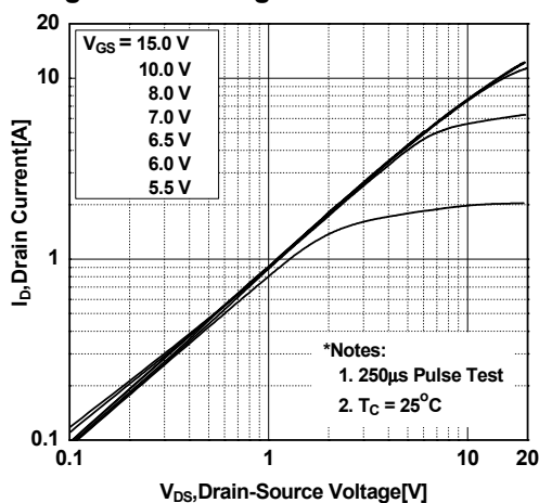
Figure 1. On-Region Characteristics
