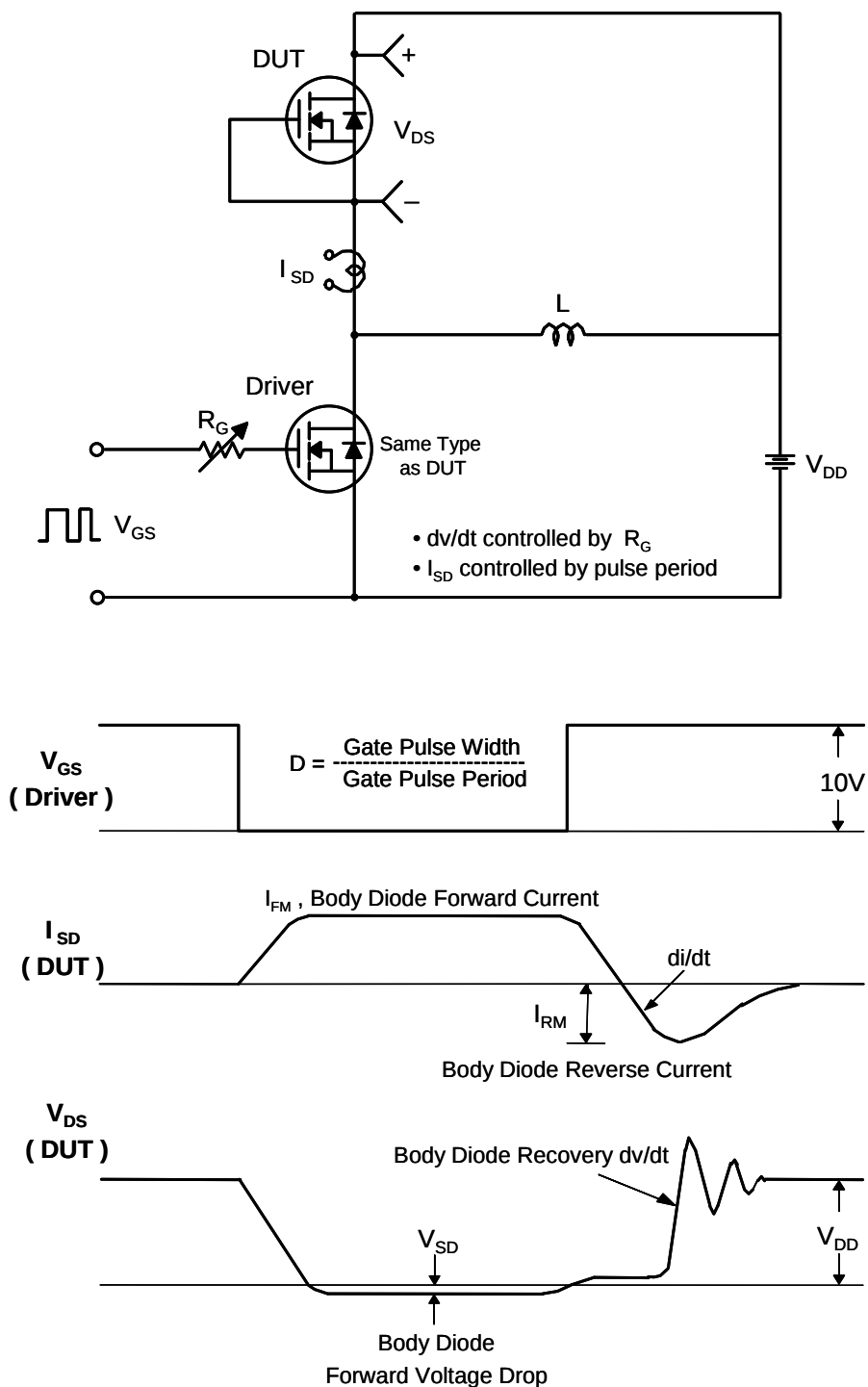
Figure 16. Unclamped Inductive Switching Test Circuit & Waveforms
