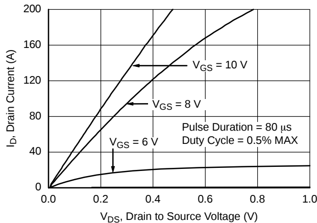
Figure 50. On-Region Characteristics
