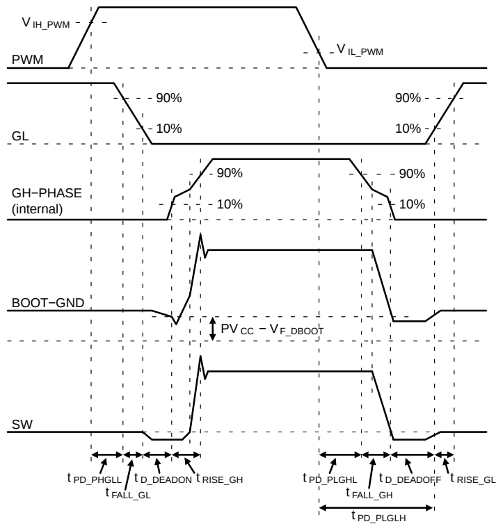
Figure 25. PWM Timing Diagram
