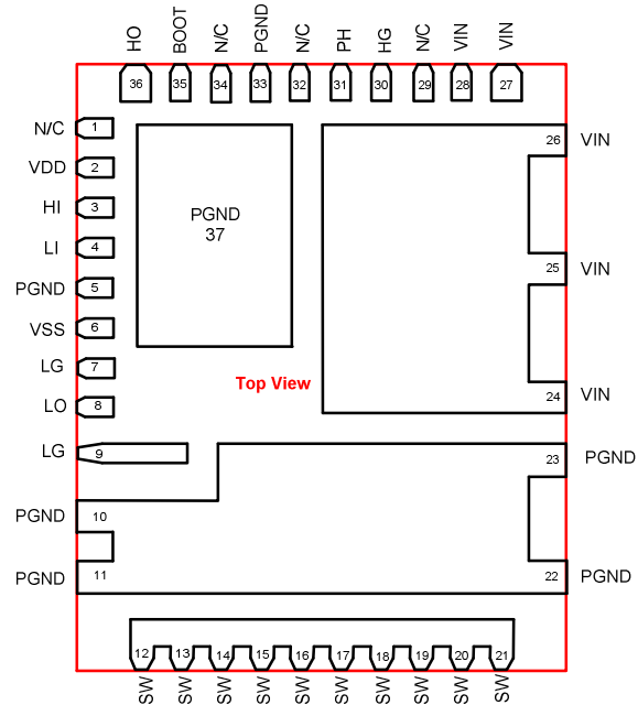
Figure 2. Pin Configuration (6.0 mm x 7.5 mm Package)
