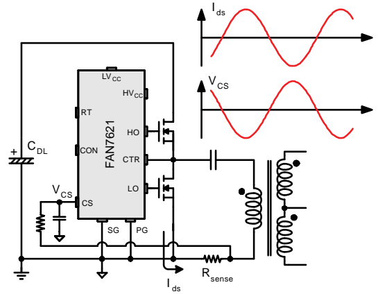
Figure 26. Full-Wave Sensing
