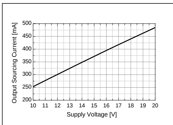
Figure 33. Output Source Current vs. Supply Voltage
