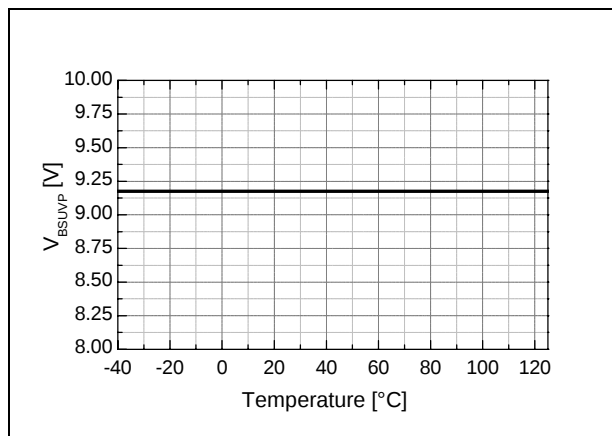
Figure 6. V_{BS} UVLO (+) vs. Temperature
