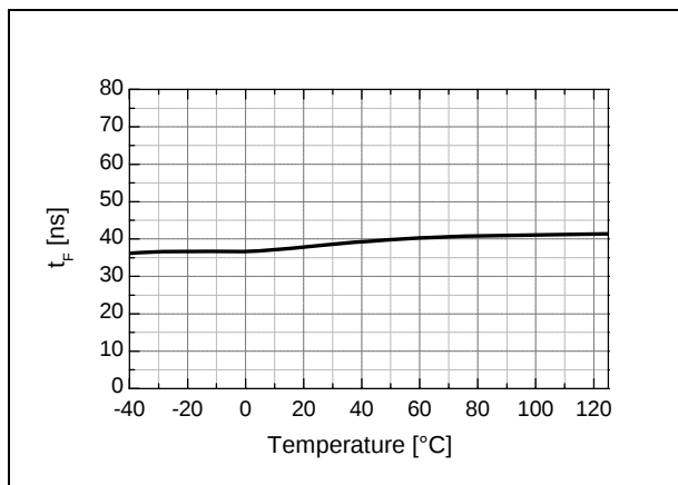
Figure 19. Falling Time vs. Temperature
