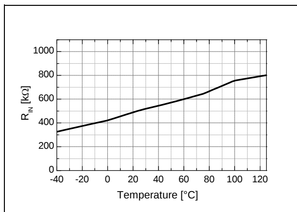
Figure 17. Logic Input Resistance vs. Temperature
