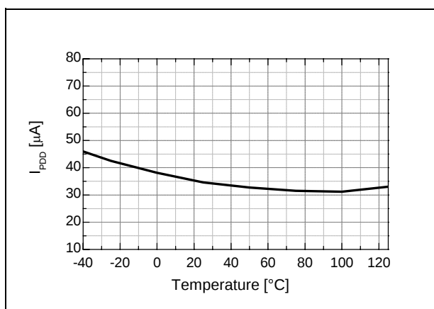
Figure 11. V_{DD} Operating Current vs. Temperature
