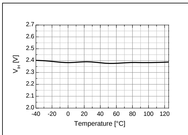
Figure 15. Logic Input High Voltage vs. Temperature
