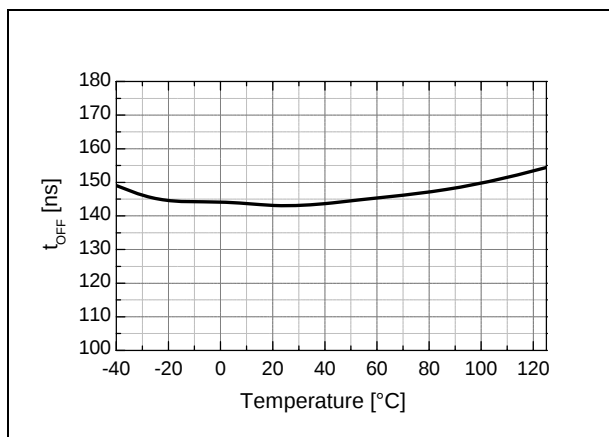
Figure 21. Turn-Off Delay Time vs. Temperature
