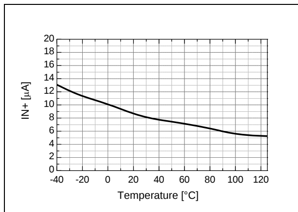
Figure 13. Logic High Input Current vs. Temperature
