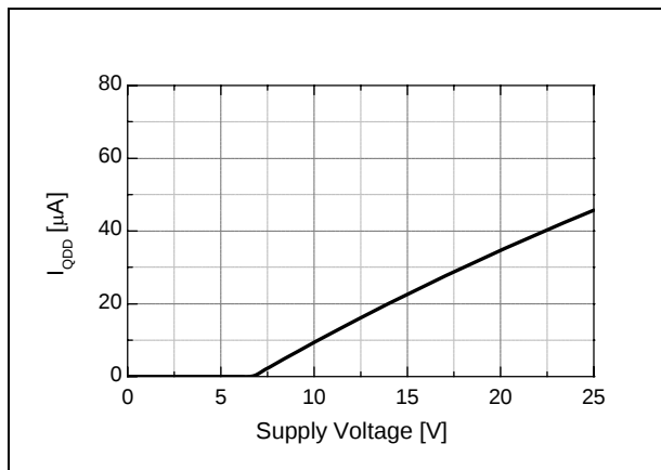
Figure 26. V_{DD} Quiescent Current vs. Supply Voltage
