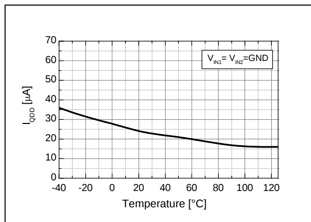
Figure 9. V_{DD} Quiescent Current vs. Temperature
