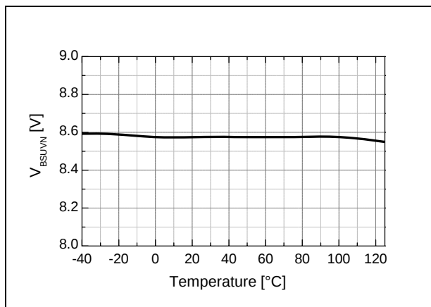
Figure 7. V_{BS} UVLO (-) vs. Temperature
