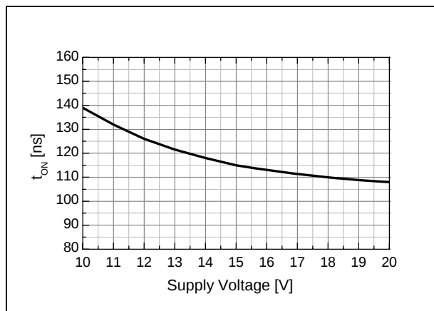
Figure 31. Turn-On Delay Time vs. Supply Voltage
