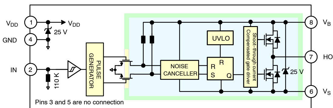
Figure 2. Block Diagram
