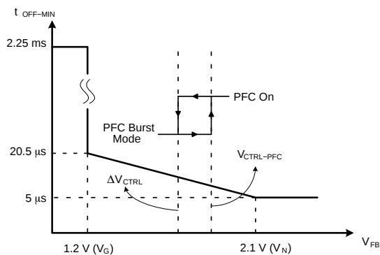
Figure 39. V_{FB} Voltage vs. t_{OFF-MIN} Time Characteristic Curve
