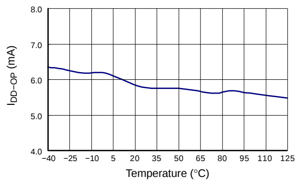
Figure 9. Operating Current
