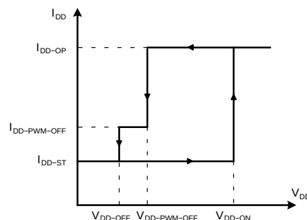
Figure 37. V_{DD} vs. I_{DD-OP} Characteristic Curve
