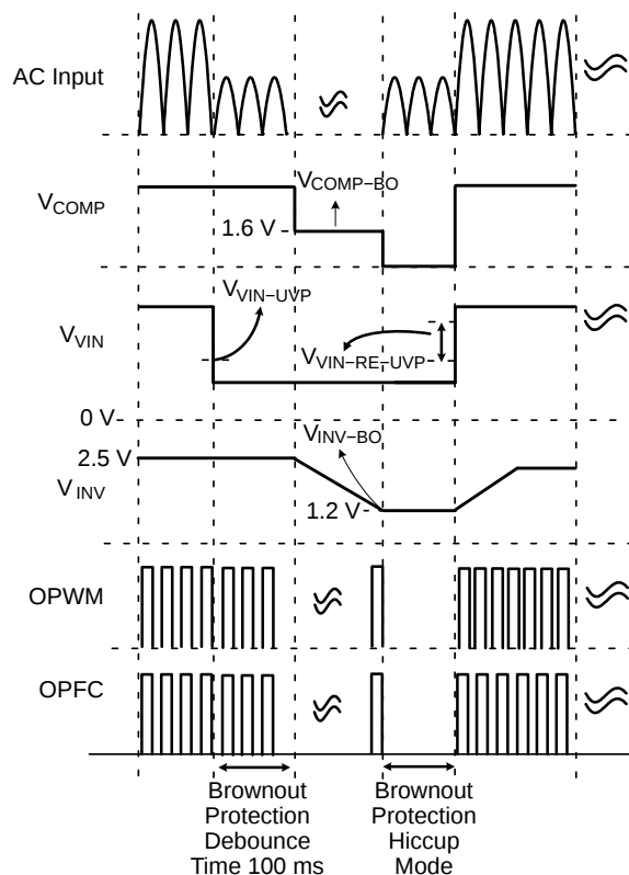
Figure 33. Operation Waveforms of Brownout / In Protection
