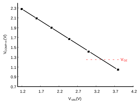
Figure 36. V_{COMP-H} Voltage vs. V_{IN} Voltage Characteristic Curve
