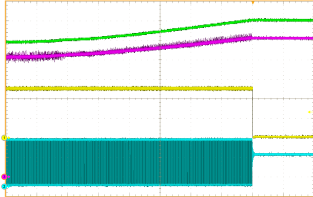
Figure 29. OVP1 at V_{FB} \geq 115\% V_{REF}
