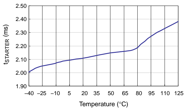
Figure 15. Start Timer ( V_{FB} < V_G )
