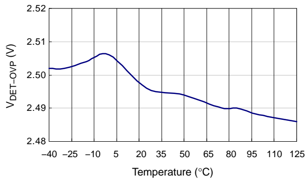
Figure 12. Comparator Reference Voltage
