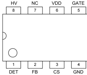
Figure 3. Pin Configuration
