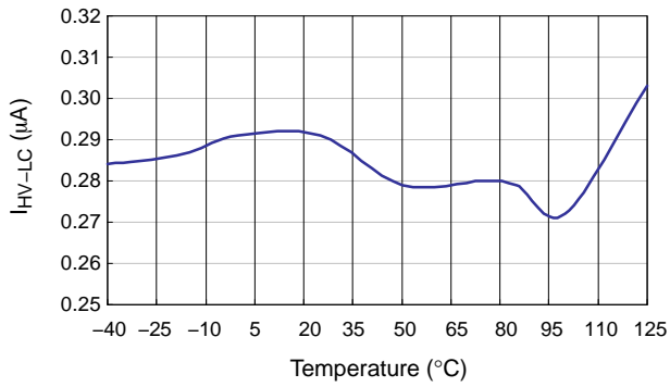
Figure 10. Leakage Current after Startup
