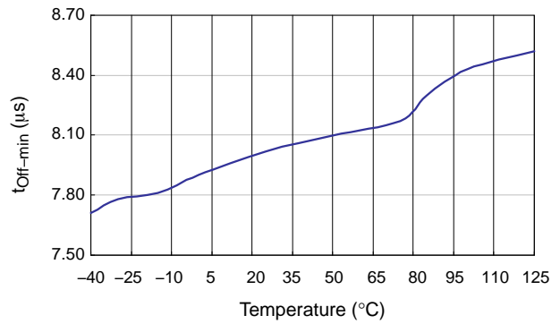
Figure 13. Minimum Off Time ( V_{FB} > V_N )
