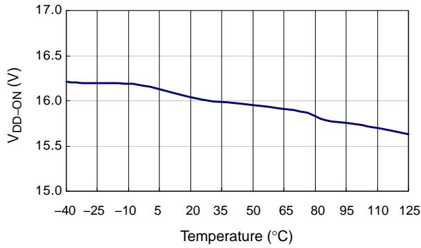
Figure 4. Turn-On Threshold Voltage
