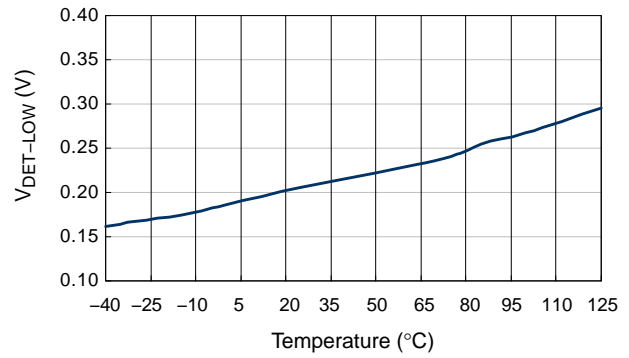
Figure 11. Lower Clamp Voltage
