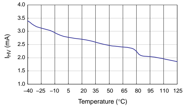
Figure 9. Supply Current Drawn from HV Pin
