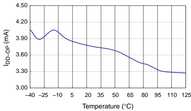
Figure 8. Operating Current
