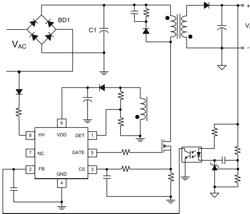
Figure 1. Typical Application
