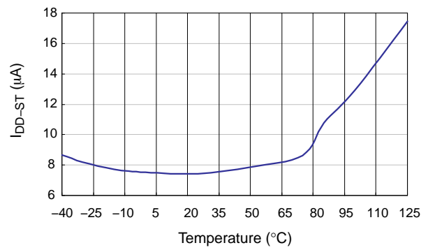
Figure 7. Startup Current
