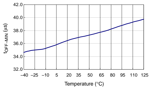
Figure 14. Minimum Off Time ( V_{FB} = V_G )
