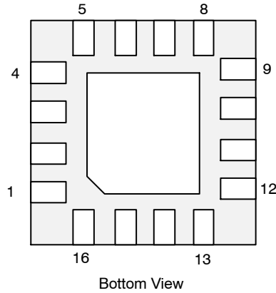
Figure 3. UQFN-16, 0.5 mm Pitch, 3 mm x 3 mm
