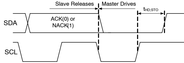
Figure 39. Stop Bit
