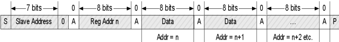
Figure 44. Multi-Byte (Sequential) Write Transaction
