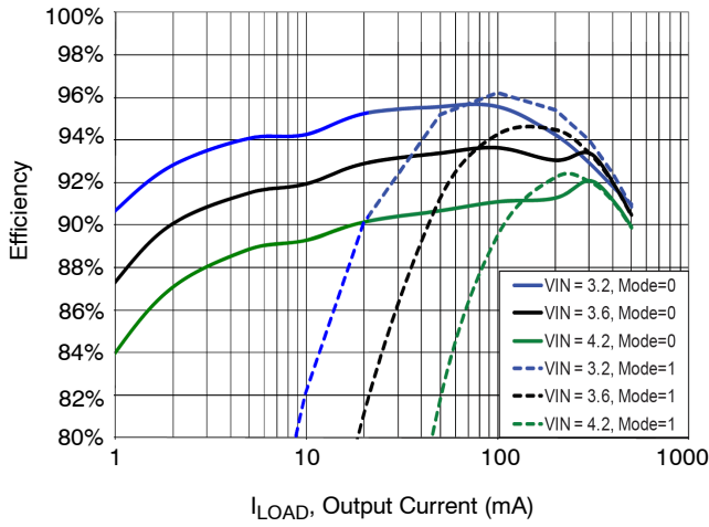
Figure 5. Efficiency vs. Load Current and Input Supply
