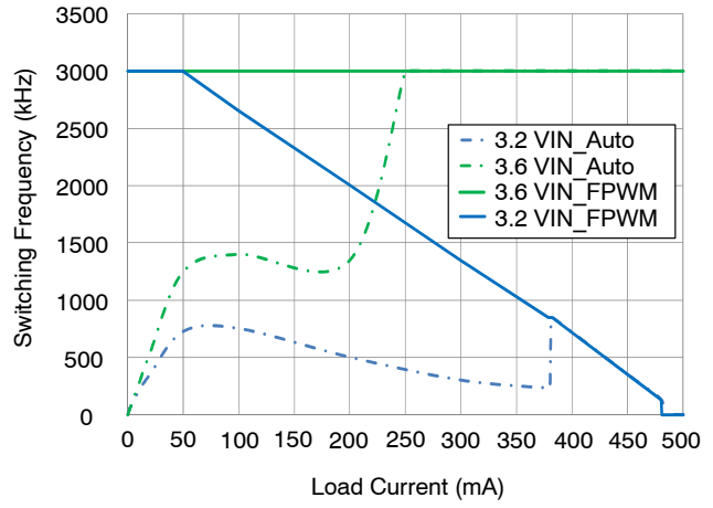
Figure 8. Effect of t_{OFF(MIN)} on Reducing Switching Frequency
