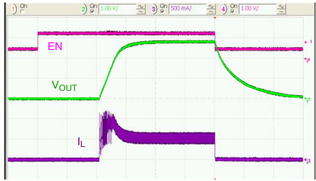
Figure 18. Startup and Shutdown through V_{EN} with 500 mA Load, 50 \mu\text{s} /div.
