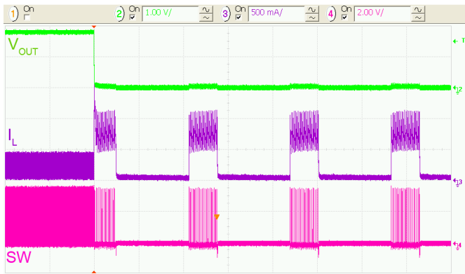
Figure 33. Metallic Short Applied at V_{OUT} , 50\ \mu\text{s/div.}
