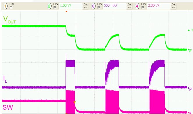
Figure 35. Over-Current Fault Response, R_{LOAD} = 1\ \Omega , 50\ \mu\text{s/div.}
