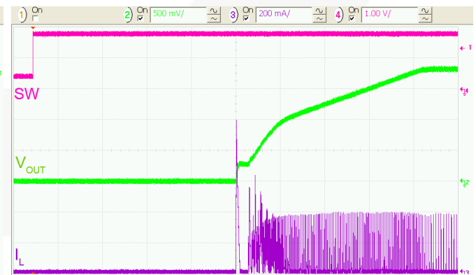
Figure 38. Soft-Start, R_{LOAD} = 50\ \Omega , 20\ \mu\text{s/div.}
